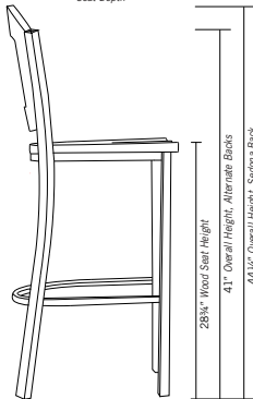
Bar Stool (Side)
